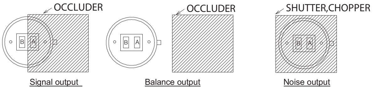
Figure 3. ZRE200GE Test Setup Block Diagram
