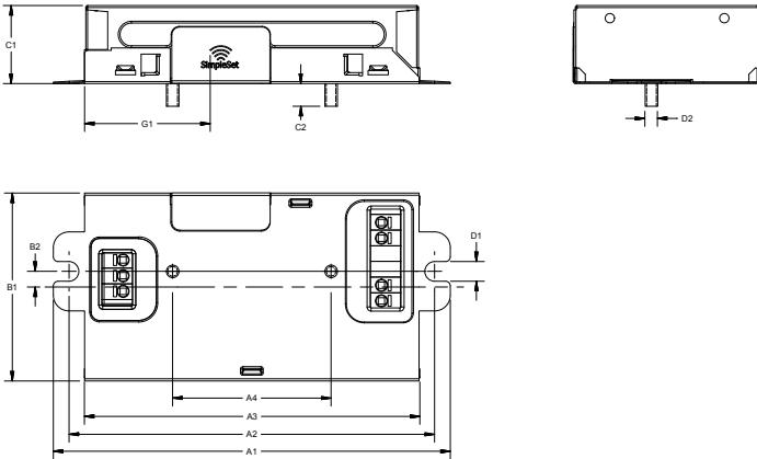
XI025C100V054BSM2 (bottom entry)
