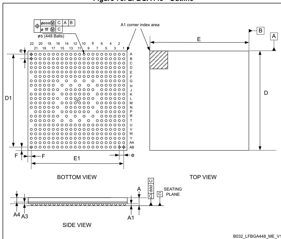
Figure 75. LFBGA448 - Outline
