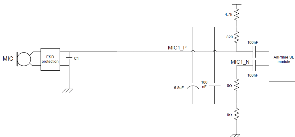
Figure 16. Example – MIC Single-Ended Connection without an LC Filter
