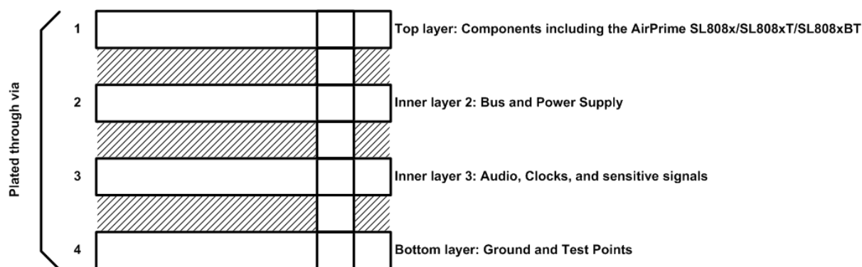
Figure 31. PCB Structure Example for the Application Board
