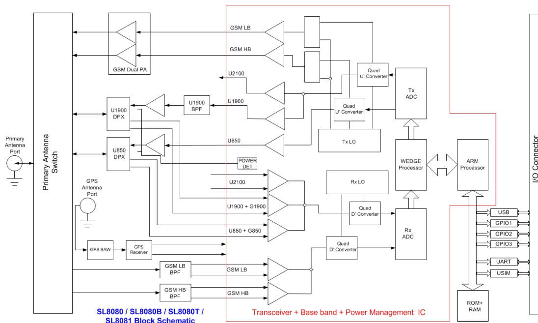
Figure 7. SL8080/SL8080B/SL8080T/SL8081 System Block
