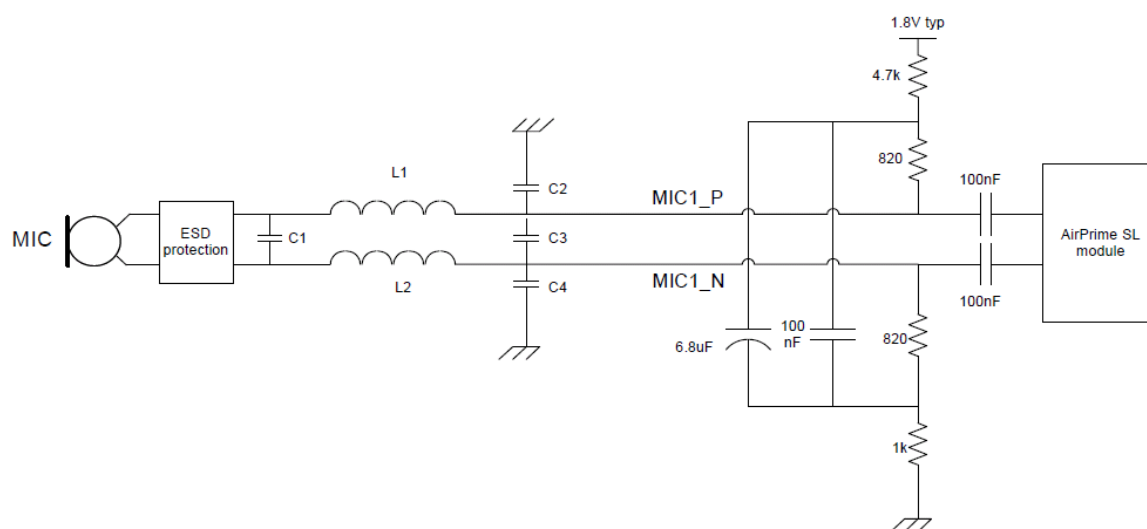
Figure 13. Example – MIC Differential Connection with LC Filter
