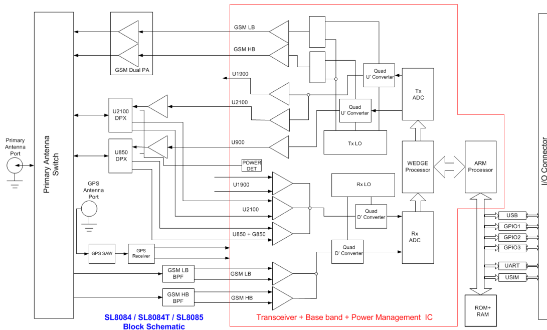
Figure 9. SL8084/SL8084T/SL8085 System Block
