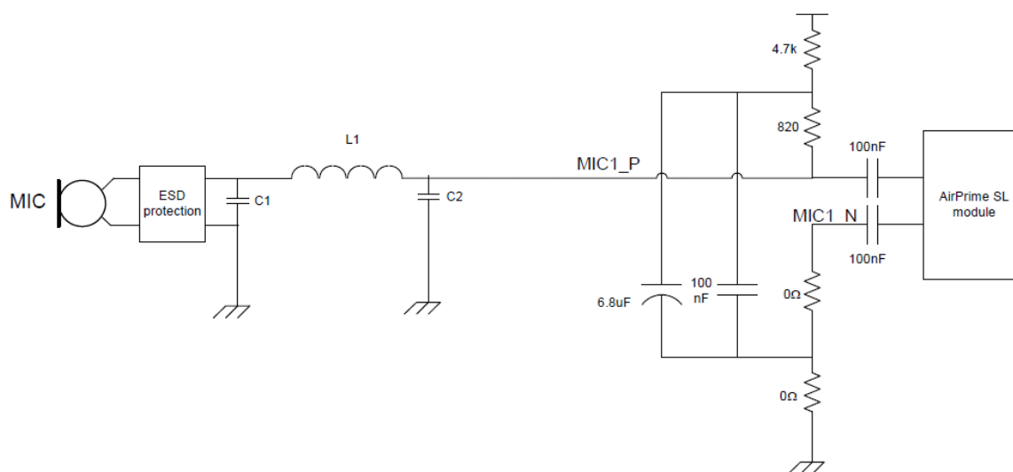
Figure 15. Example – MIC Single-Ended Connection with LC Filter
