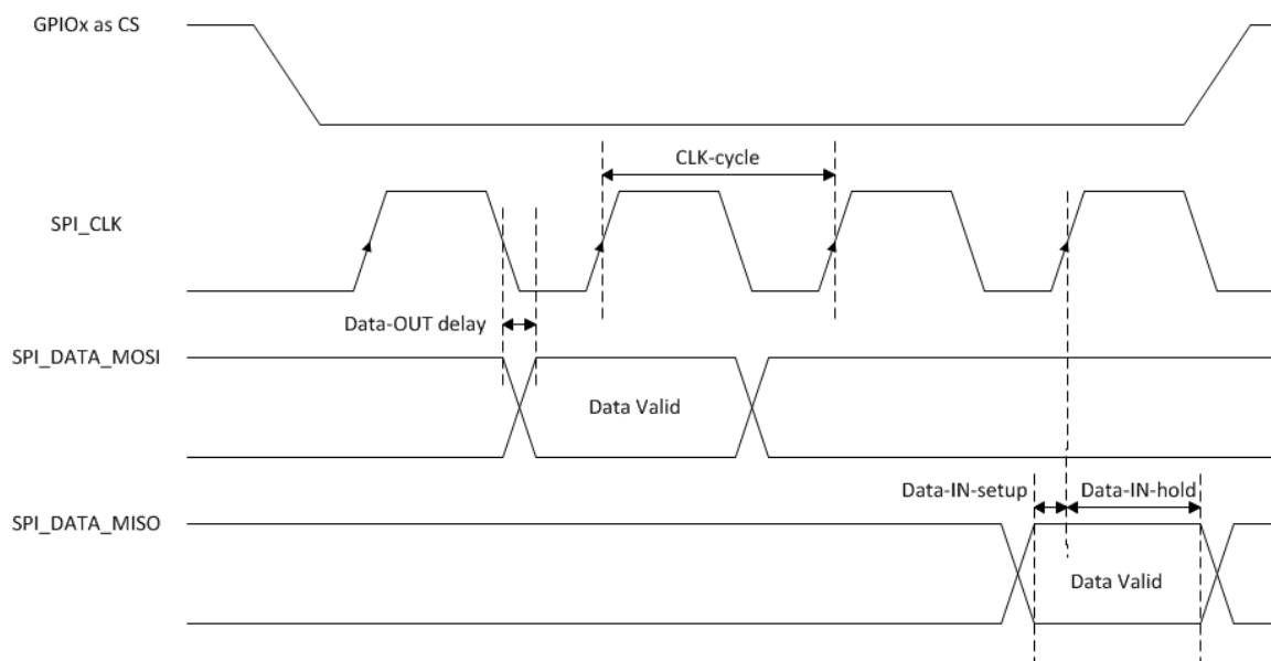
Figure 11. SPI Timing Diagram (Mode 0, Master, 4wires)
