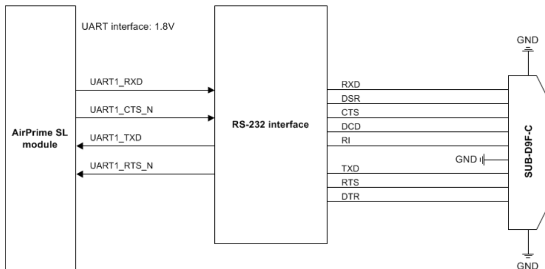
Figure 37. 4-wire Main Serial Interface (UART1) for SL808x, SL808xT or SL808xBT
