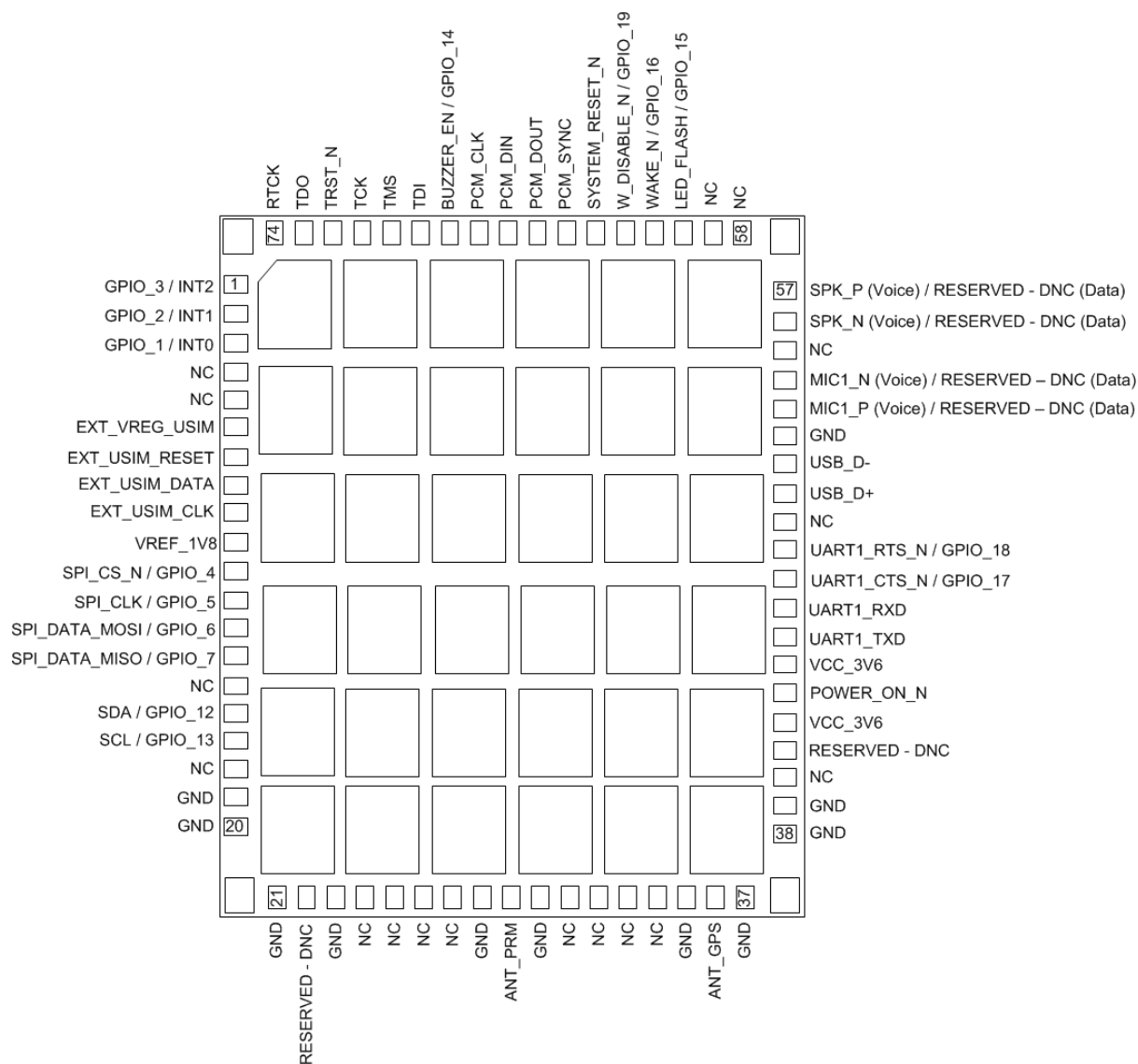
Figure 10. SL808x, SL808xT and SL808xBT Device Pinouts 2
