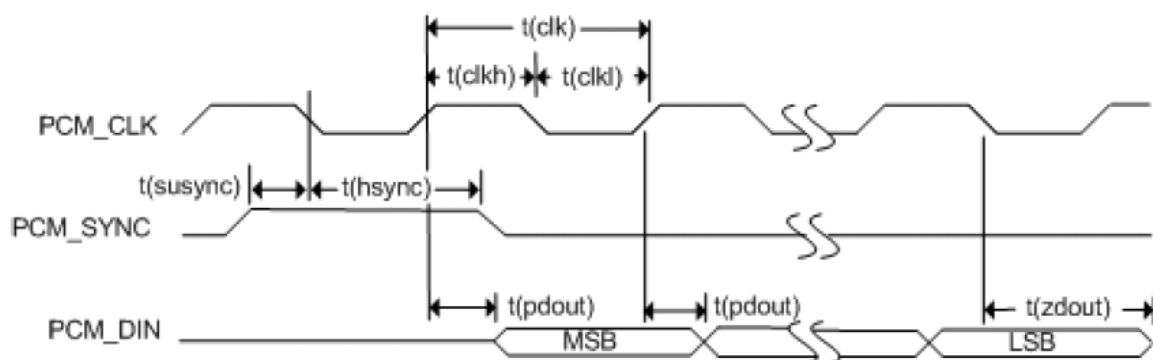
Figure 22. Timing Diagram – SL808x, SL808xT and SL808xBT to External PCM_CODEC
