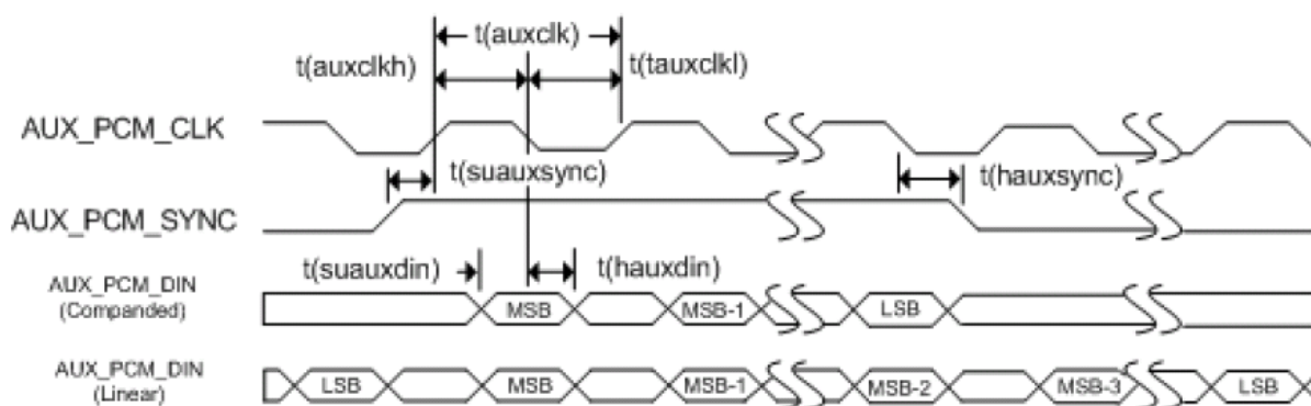
Figure 24. Timing Diagram – AUX_PCM_CODEC to SL808x, SL808xT and SL808xBT
