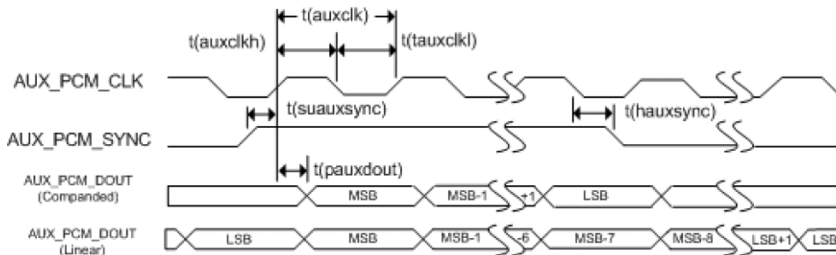
Figure 25. Timing Diagram – SL808x, SL808xT and SL808xBT to AUX_PCM_CODEC
