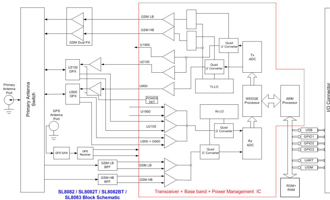
Figure 8. SL8082/SL8082T/SL8082BT/SL8083 System Block
