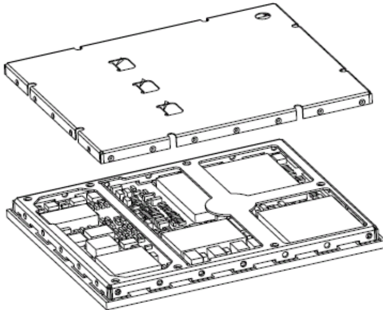
Figure 2. Exploded View
