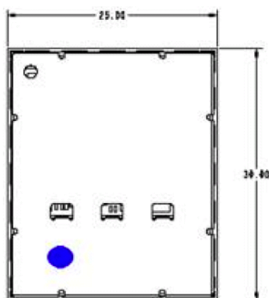
Figure 35. Recommended Thermocouple Location
