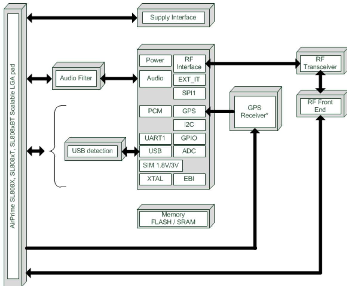
Figure 1. Functional Architecture
