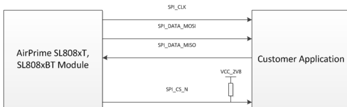
Figure 12. Example of a 4-wire SPI Bus Application
