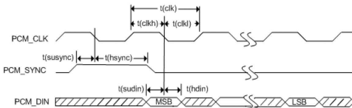
Figure 21. Timing Diagram – PCM_CODEC to SL808x, SL808xT and SL808xBT
