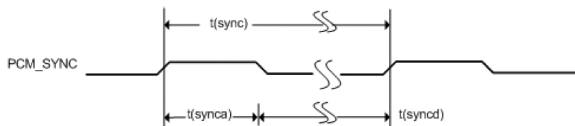
Figure 20. Timing Diagram – Short Frame Sync (PCM_SYNC)
