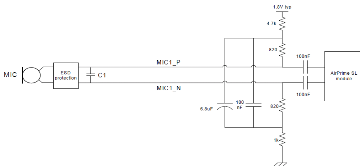
Figure 14. Example – MIC Differential Connection without an LC Filter
