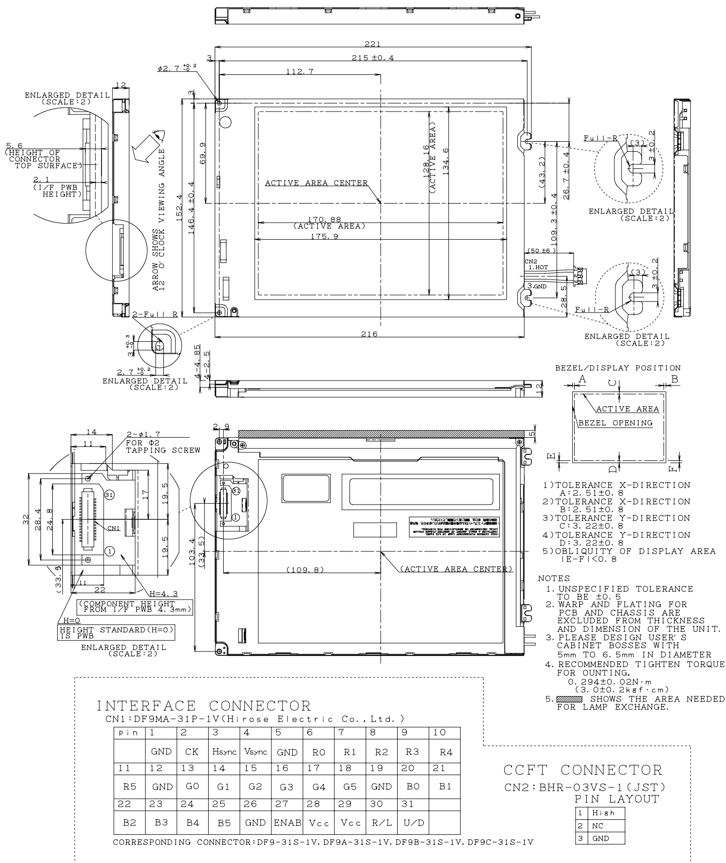
FIG1. OUTLINE DEMENSIONS LQ084V1DG41
