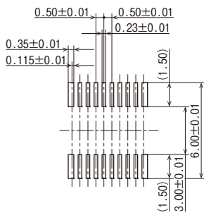
Recommended metal mask pattern Metal mask thickness: When 150\mu\text{m} (Opening area ratio: 69%)
