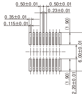
Recommended metal mask pattern Metal mask thickness: When 120\mu\text{m} (Opening area ratio: 87%)
