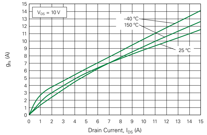
Fig. 2. Typical Transconductance
