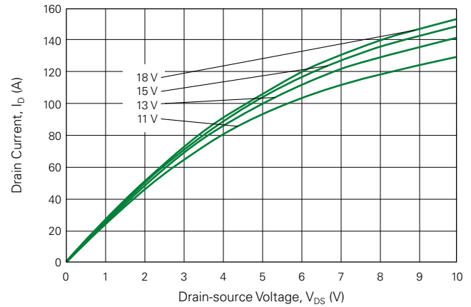
Fig. 4. Typical Output Characteristics @ T_{vj} = 150 °C
