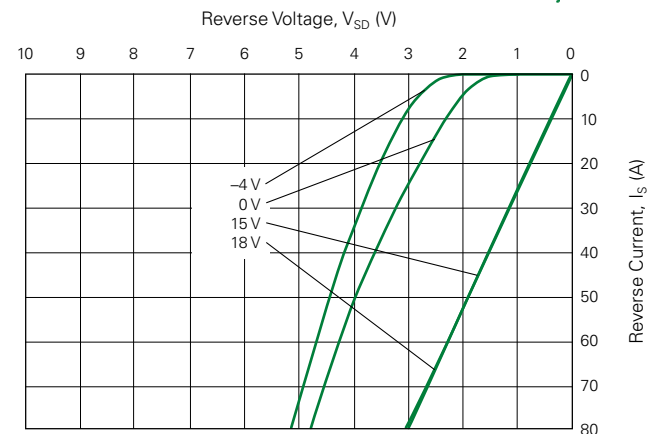
Fig. 12. Typical Reverse Conduction Characteristics @ T_{vj} = 150\text{ °C}
