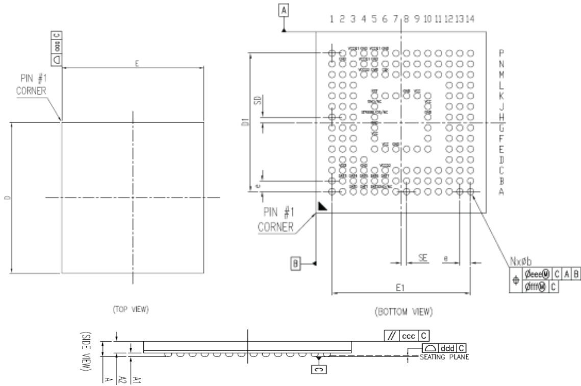
Figure 2 – Package Dimensions
