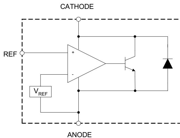
Figure 3. Functional Block Diagram of AZ431-A
