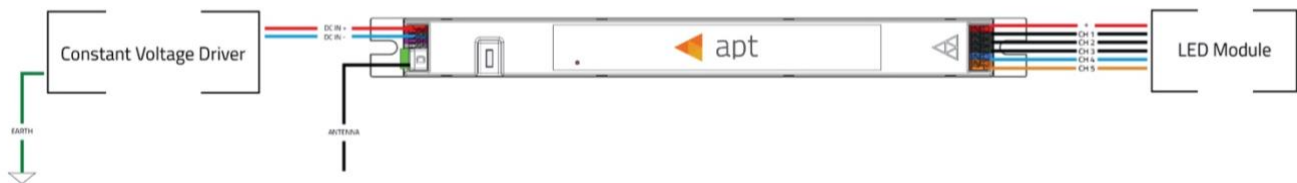
Figure 4 - APT-CV5-VWC Wireless Communication Configuration
