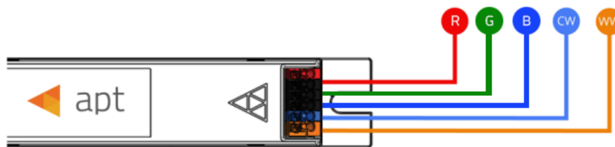
Figure 3 - Wiring APT-CV5-VA-LN to RGBWW LED Module
