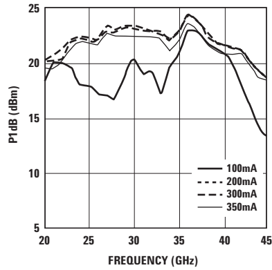
Figure 8. Output Power ( P_{-1dB} ) and Drain Current, V_{DD}=4.5V .
