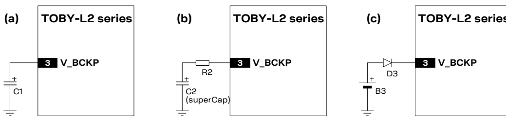
Figure 41: Real time clock supply (V_BCKP) application circuits: (a) using a 100 μF capacitor to let the RTC run for ~80 s after VCC removal; (b) using a 70 mF capacitor to let RTC run for ~15 hours after VCC removal; (c) using a non-rechargeable battery
