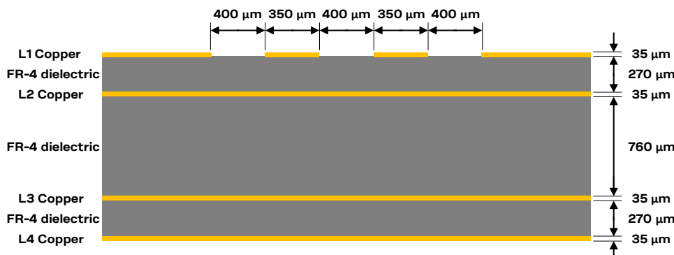
Figure 55: Example of USB line design, with Z_0 close to 90 \Omega and Z_{CM} close to 30 \Omega , for the described 4-layer board layup
