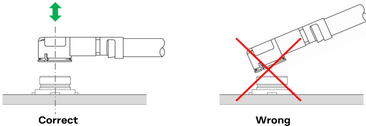
Figure 71: Precautions during RF connector mating
