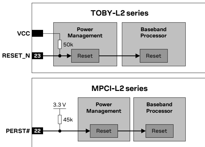
Figure 17: TOBY-L2 and MPC-L2 series RESET_N and PERST# input equivalent circuit description
