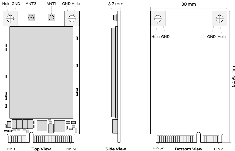
Figure 70: MPC-L2 series mechanical description (top, side and bottom views)
