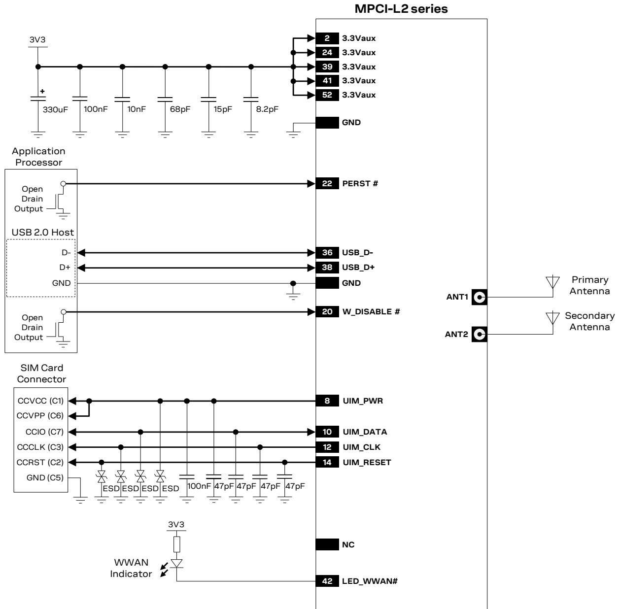
Figure 76: Example of schematic to integrate a MPCl-L2 series module in an application board, using all the interfaces
