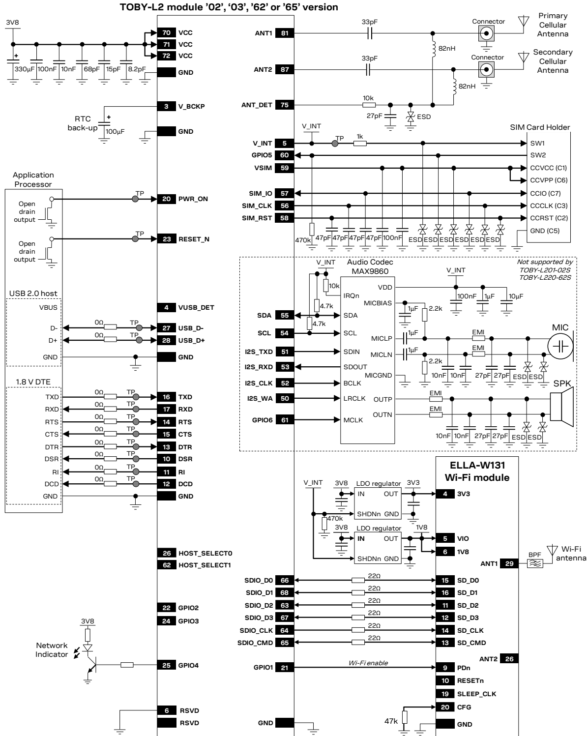
Figure 75: Example schematic integrating TOBY-L2 module '02', '03', '62', or '65' version in an application using all interfaces
