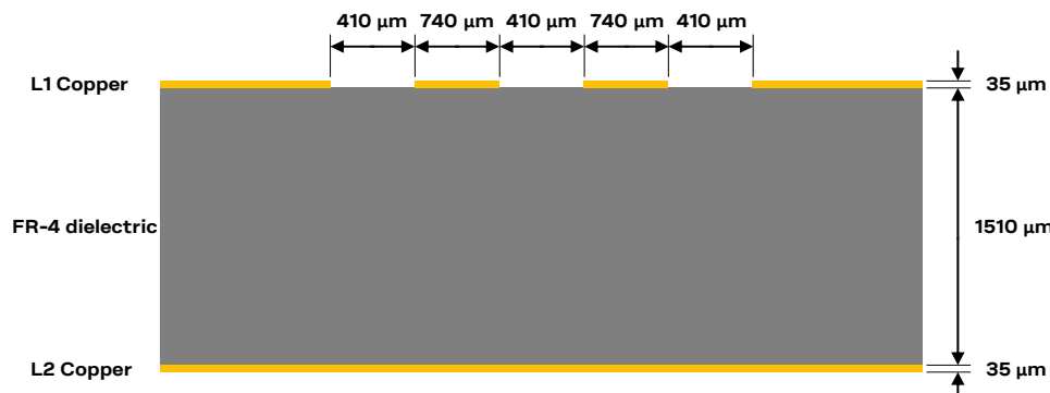
Figure 56: Example of USB line design, with Z_0 close to 90 \Omega and Z_{CM} close to 30 \Omega , for the described 2-layer board layup
