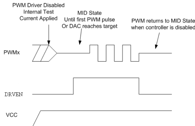
Figure 3. Soft-Start Sequence
