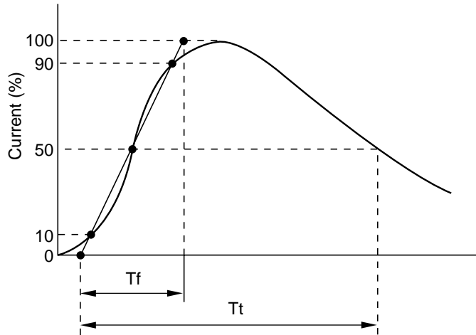
(Impulse Current Wave Form)
