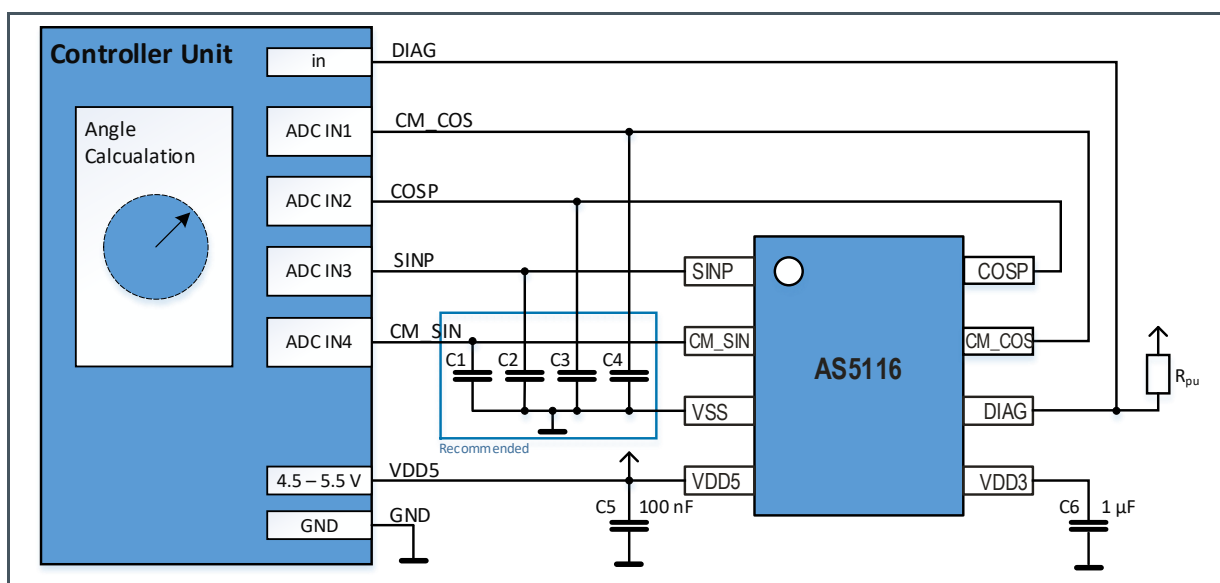
Figure 34: AS5116A – Wiring Diagram, Single Ended Output Mode
