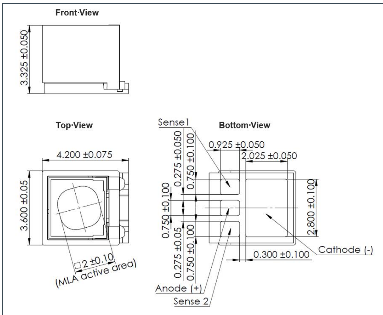
Figure 11: Package Dimensions
