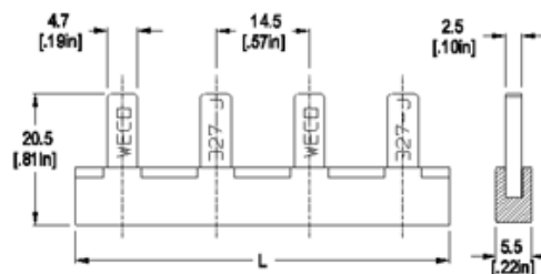
Dimensions: mm (in.)
