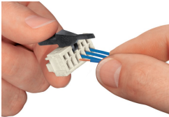
Inserting a conductor via operating lever.
