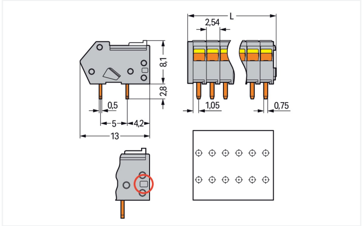
Dimensions in mm L = (pole no. x pin spacing) + 1.5 mm A groove at the back of the terminal strip indicates the 2.54 mm pin spacing (red circle).
