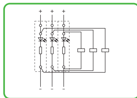
Voltage indication
