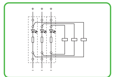
Voltage indication
