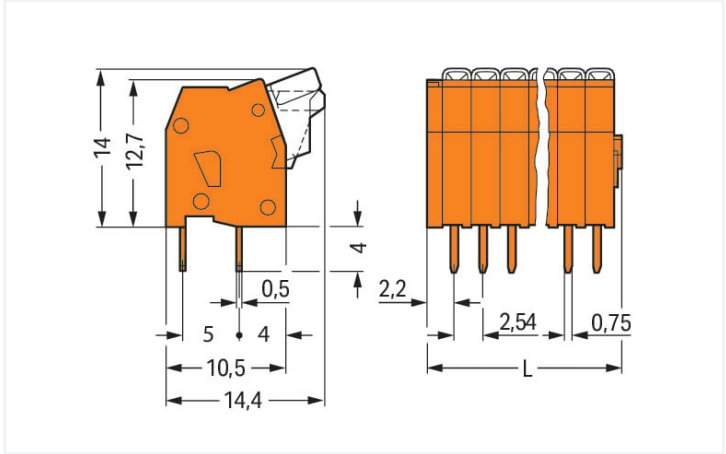
Dimensions in mm L = (\text{pole no.} \times \text{pin spacing}) + 2.2 \text{ mm}
