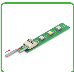
Inserting solid conductors via push-in termination.
