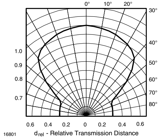
Fig. 12 - Directivity
