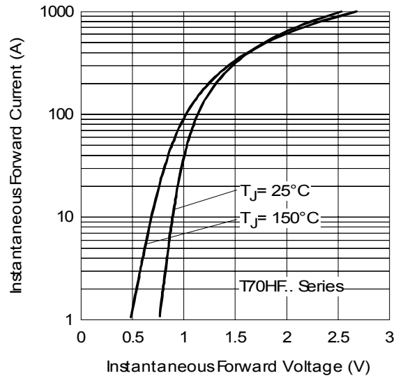
Fig. 26 - Forward Voltage Drop Characteristics
