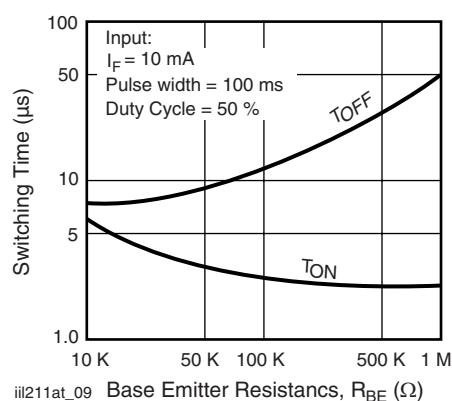
Fig. 9 - Typical Switching Characteristics vs. Base Resistance (Saturated Operation)
