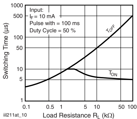
Fig. 10 - Typical Switching Times vs. Load Resistance
