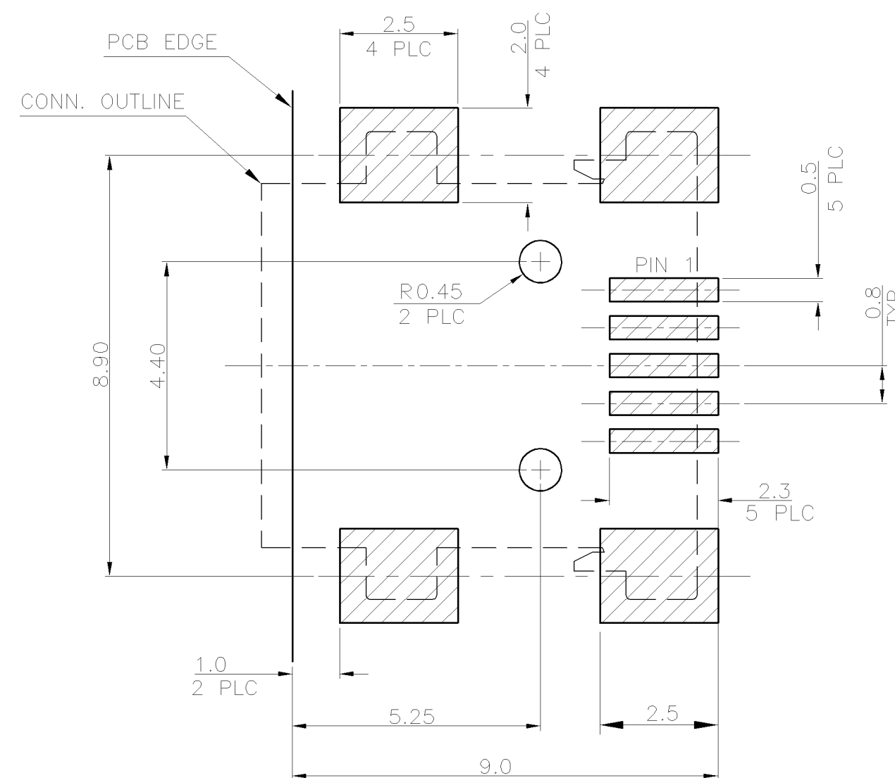
RECOMMENDED PCB LAYOUT (MOUNTING SIDE). (THICKNESS=1.6mm) (TOLERANCE=±0.05MM)
