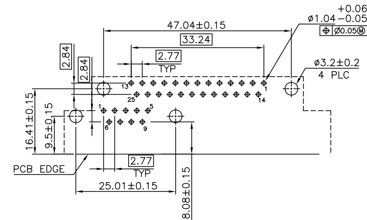
RECOMMENDED P.C.B. LAYOUT P.C.B. THICKNESS=1.6mm
