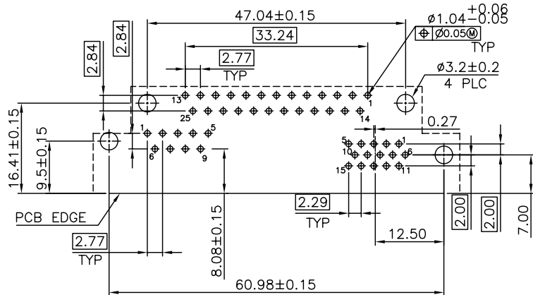
RECOMMENDED P.C.B. LAYOUT P.C.B. THICKNESS=1.6mm
