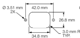
Panel cutout (front mount) Tolerance \pm 0.13 mm
