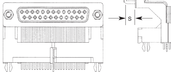
High-Rise 25 Position HD-20 Receptacle
