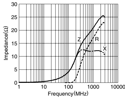
MMZ1608D500C
