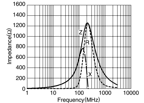
MMZ1608D100C
