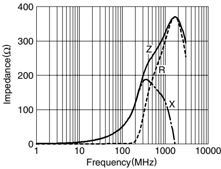
MMZ1608D500C
