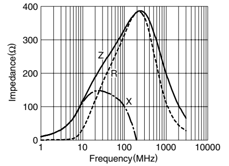
MMZ1608Y150B
