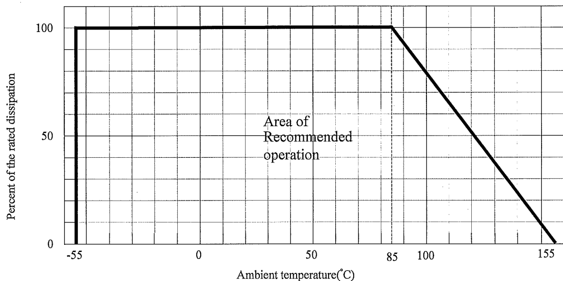
Fig. 2 Derating curve
