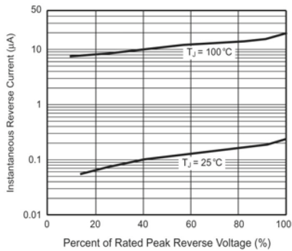
Figure 4. Typical Reverse Leakage Characteristics Per Leg
