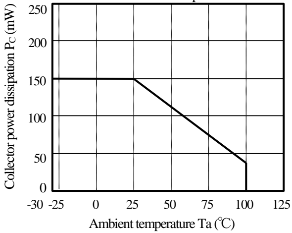
(Fig.5) Collector power dissipation vs. ambient temperature
