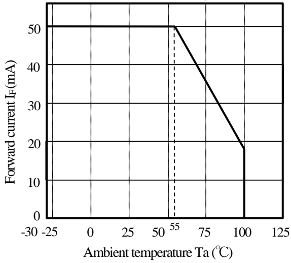
(Fig.3) Forward current vs. ambient temperature
