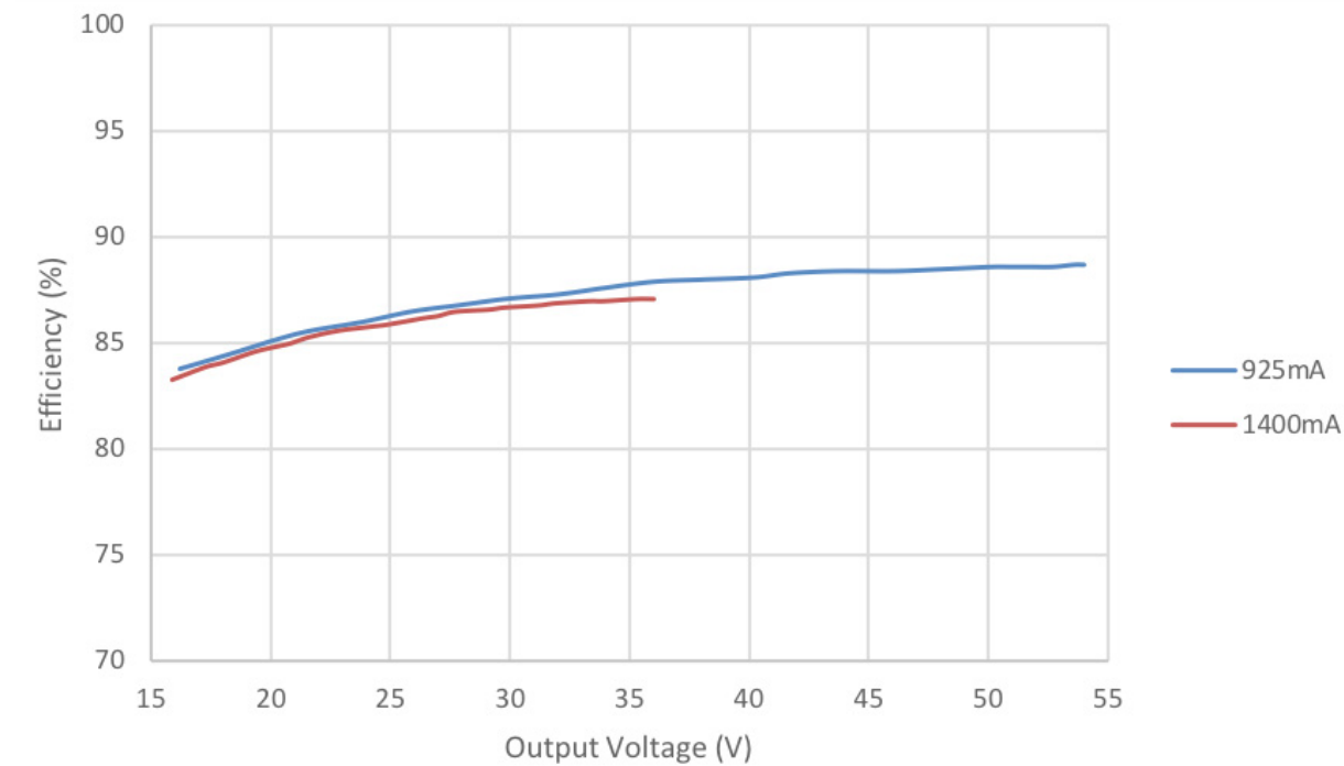
Efficiency Vs. Output Voltage at 120Vac
