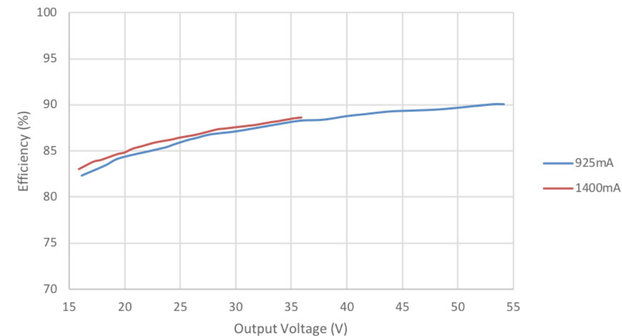
Efficiency Vs. Output Voltage at 277Vac
