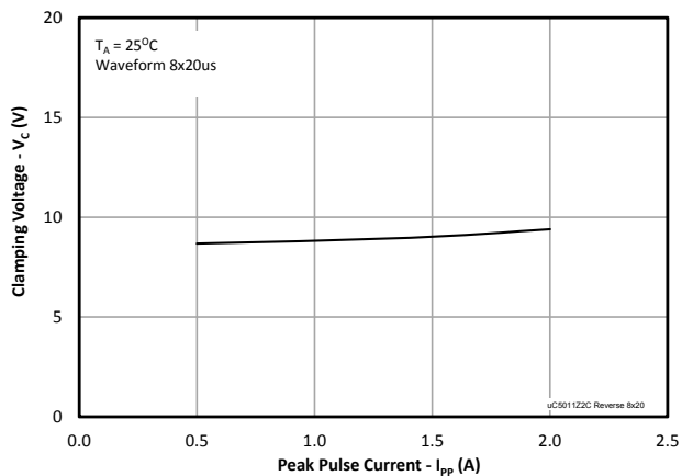
Clamping Voltage vs. Peak Pulse Current ( t_p=8/20\mu\text{s} )
