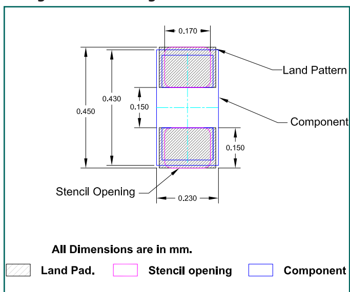
Figure 2 - Mounting Pattern - 0.050mm Stencil
