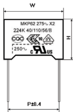
P≥15.0mm and C_R \leq 1.0\mu F
