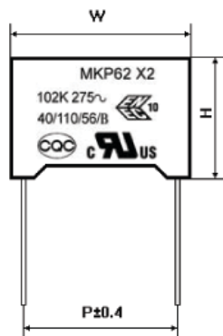
P=7.5 or 10.0mm
