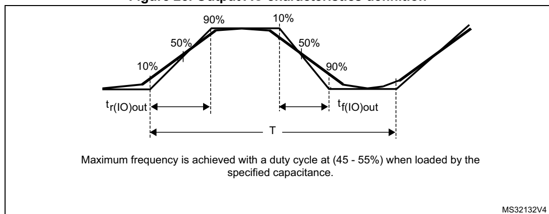
Figure 25. Output AC characteristics definition
