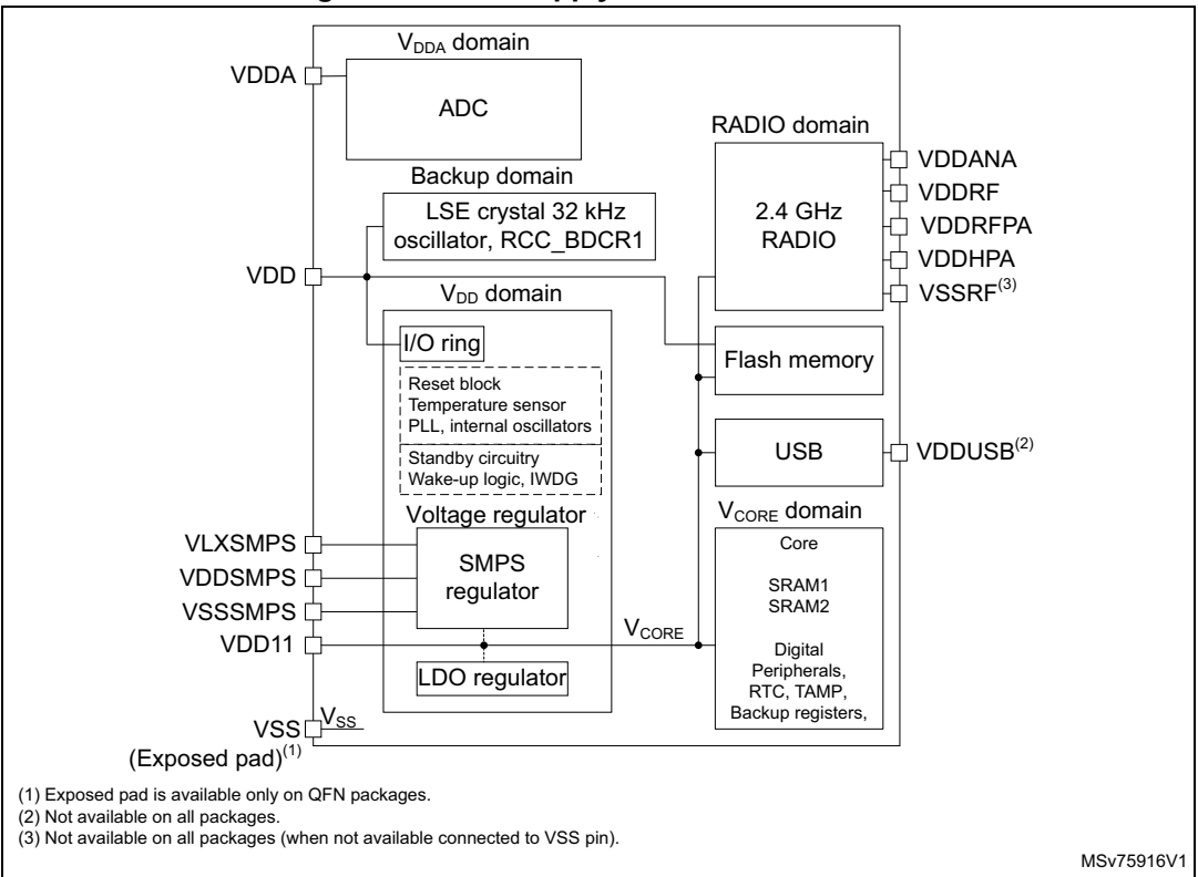
Figure 3. Power supply overview with SMPS
