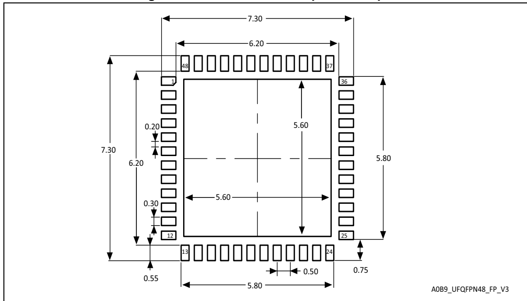
Figure 14. UFQFPN48 – Footprint example
