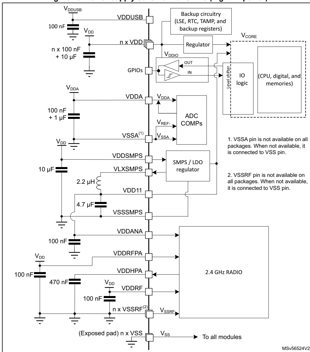
Figure 20. Power supply scheme with SMPS (high RF power)
