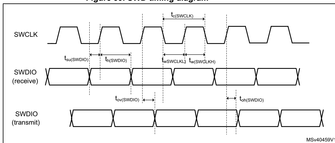
Figure 39. SWD timing diagram
