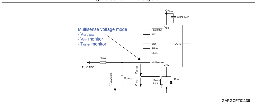
Figure 38: GND voltage shift
