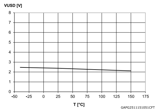
Figure 22: Undervoltage shutdown
