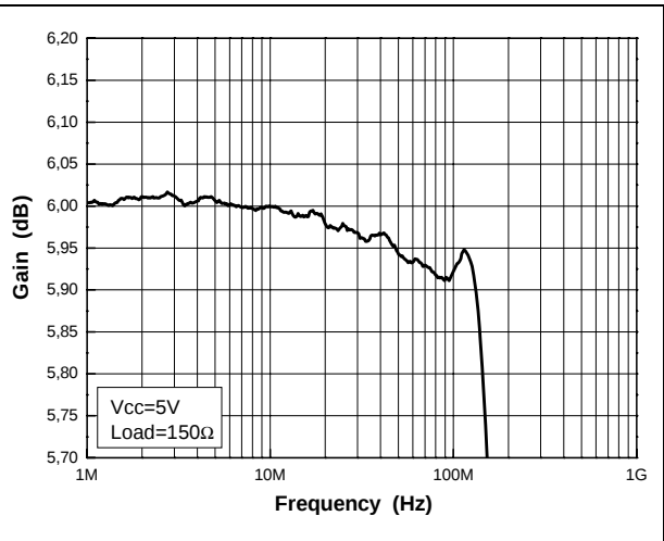
Figure 2. Gain flatness
