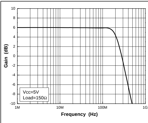
Figure 1. Frequency response
