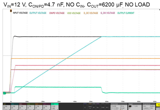
Figure 24. Startup by V_{IN} ( C_{OUT} = 6200 \mu F , no load)
