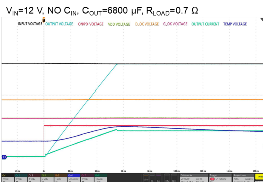
Figure 28. Start-up by ON/PD ( I_{OUT} = 15 A , C_{OUT} = 6800 \mu F )
