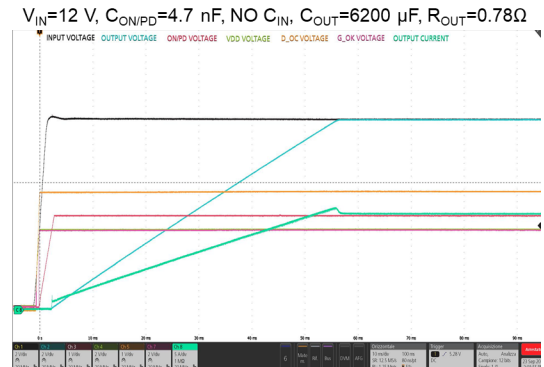
Figure 25. Startup by V_{IN} ( C_{OUT} = 6200 \mu F , 15 A, res. load)
