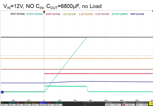
Figure 26. Startup by ON/PD (no load)
