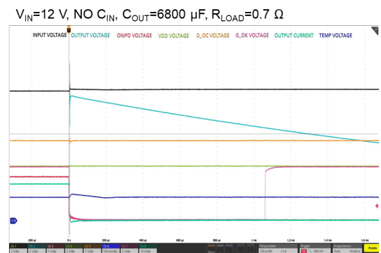
Figure 29. Shutdown by ON/PD ( I_{OUT} = 15 A , C_{OUT} = 6800 \mu F )
