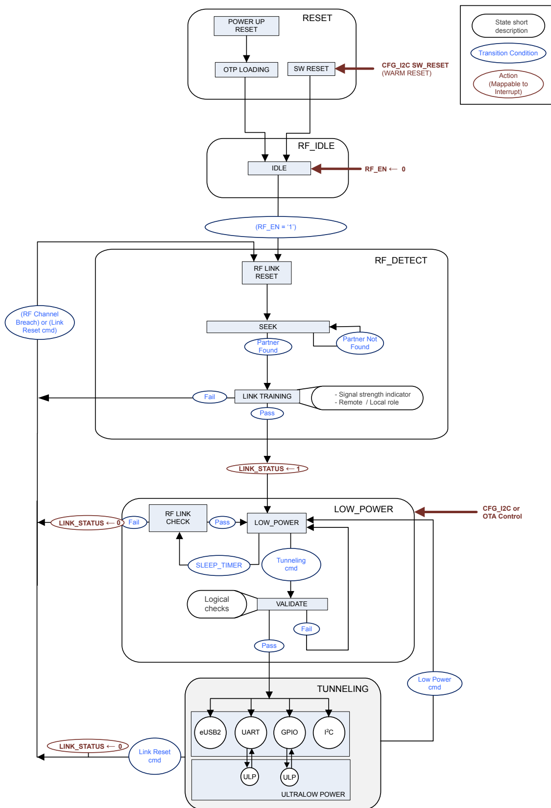
Figure 16. ST60A3H1 state machine
