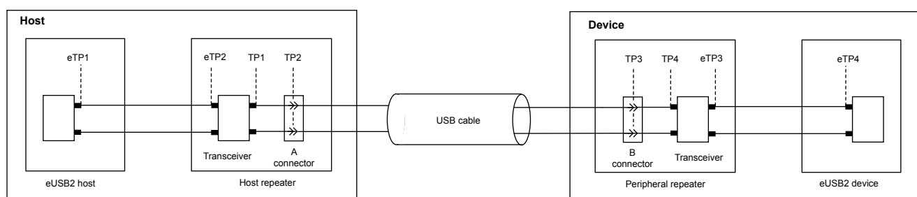
Figure 23. Measurement plane for repeater mode
