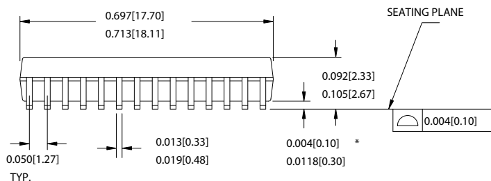
Figure 14. 28-Pin (330 mil) SOIC (51-85058)
