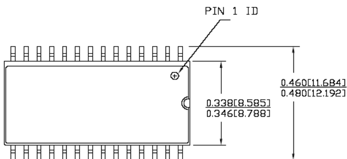
Figure 14. 28-Pin (330 mil) SOIC (51-85058)
