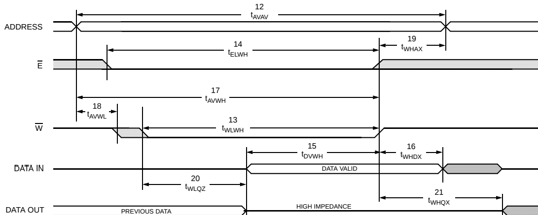
Figure 8. SRAM WRITE Cycle #1: \overline{W} Controlled [8,9]
