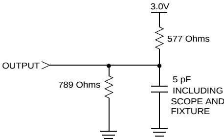
Figure 5. AC Output Loading for Tristate Specifications ( t_{HZ} , t_{LZ} , t_{WLQZ} , t_{WHQZ} , t_{GLQX} , t_{GHQZ} )
