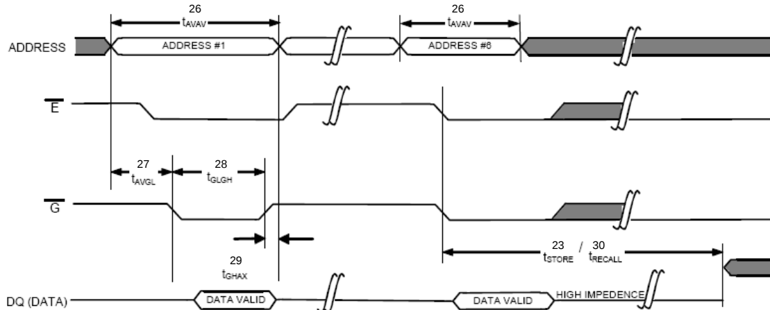
Figure 12. Software STORE/RECALL CYCLE: \overline{G} Controlled [14]
