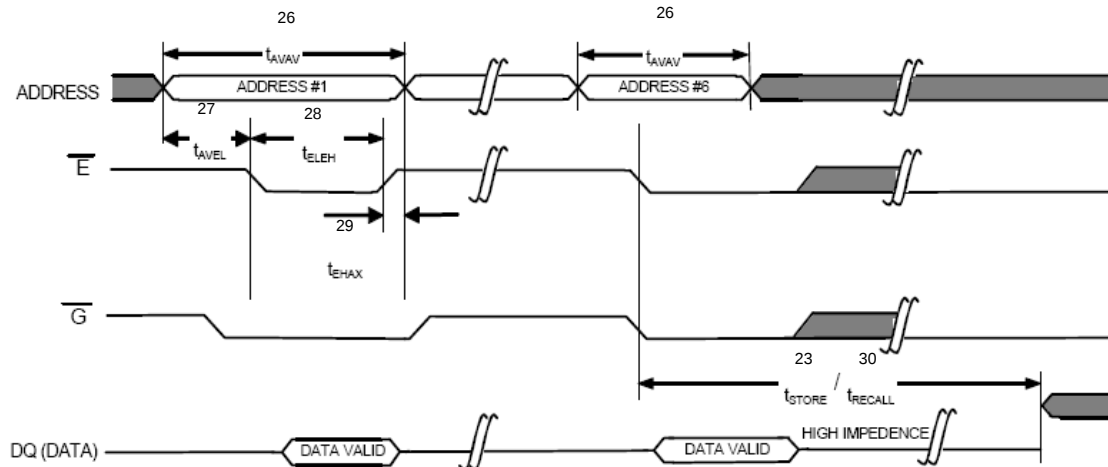
Figure 11. Software STORE/RECALL CYCLE: \overline{E} Controlled [14]
