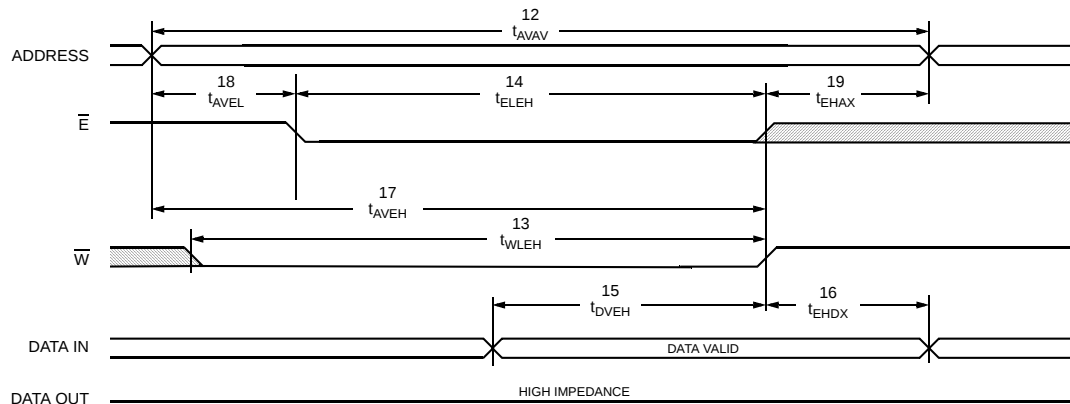
Figure 9. SRAM WRITE Cycle #2: \overline{E} Controlled [8,9]
