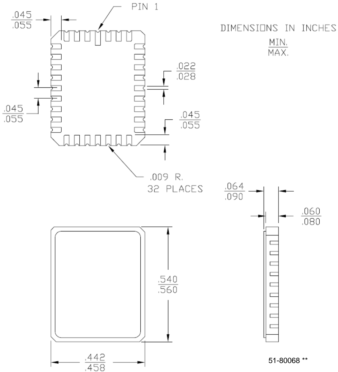
Figure 17. 32-Pin 450 mil Ceramic LCC (51-80068)
