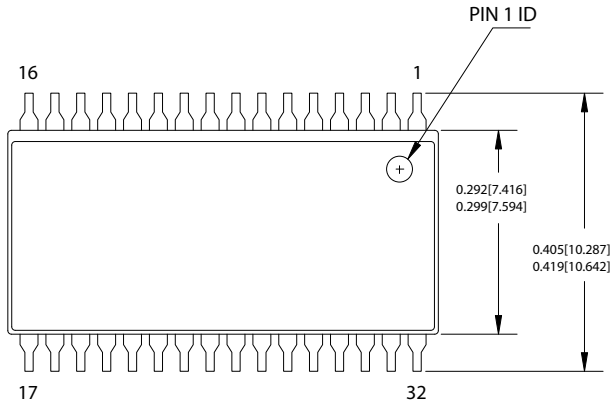
Figure 15. 32-Pin 300 mil SOIC Gull Wing (51-85127)
