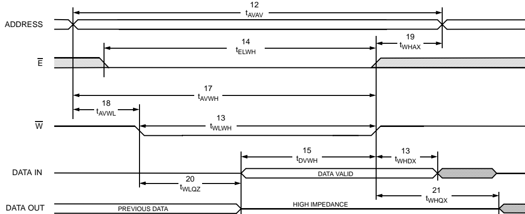
Figure 6. SRAM Write Cycle 1: \overline{W} Controlled [10, 11]
