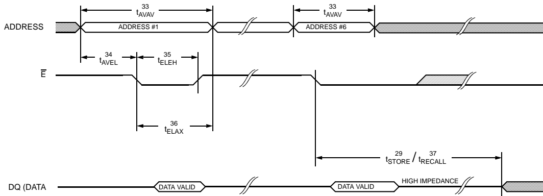
Figure 10. E Controlled Software STORE/RECALL Cycle [21]
