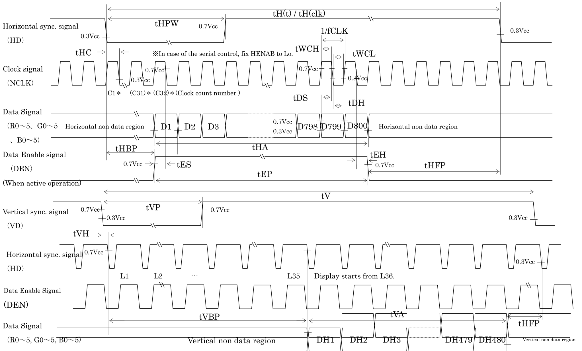
Fig. 2: Input signal timing chart
