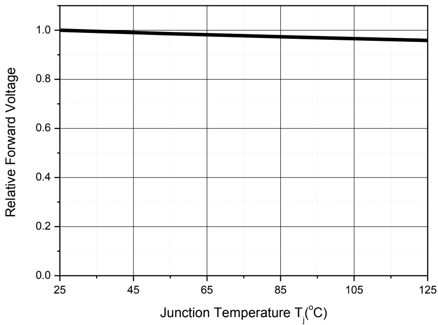
Fig 7. Junction Temperature vs. Relative Forward Voltage, I_F=65mA
