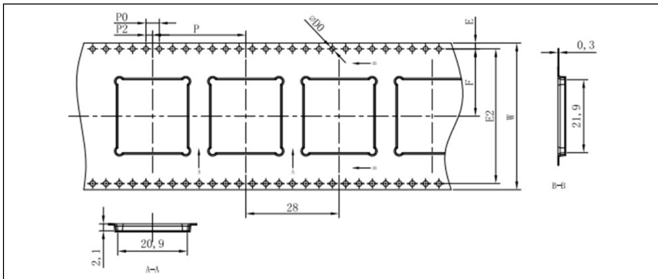
Figure 8. Packing Details
