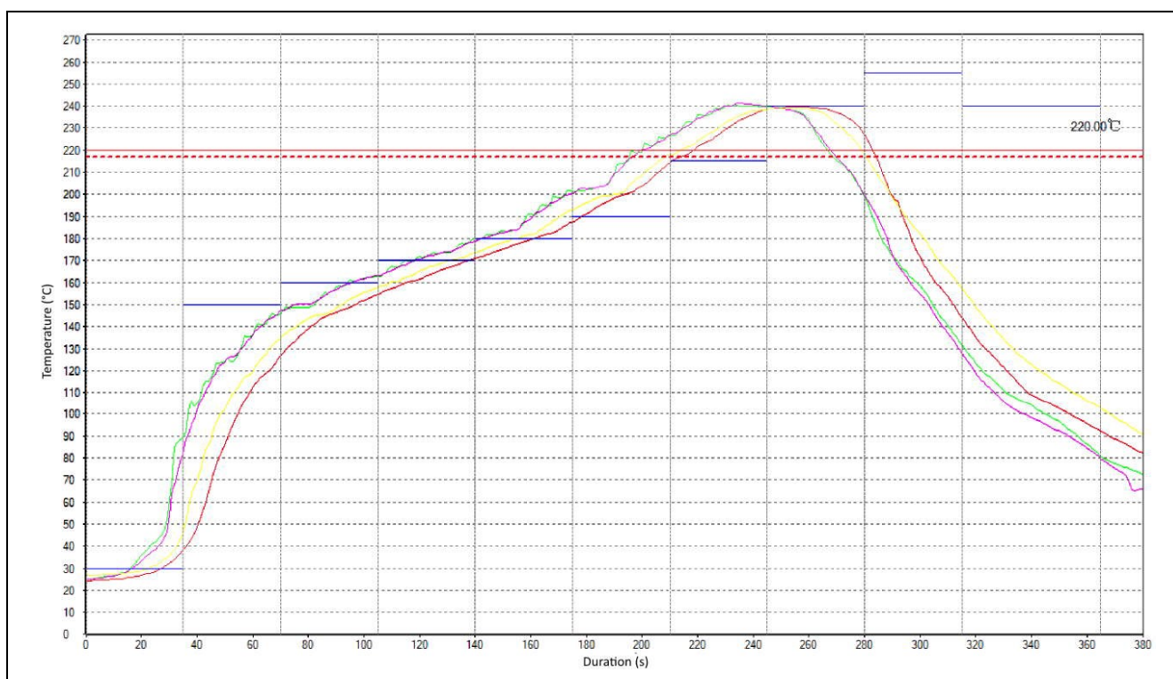
Figure 9. Reflow Profile
