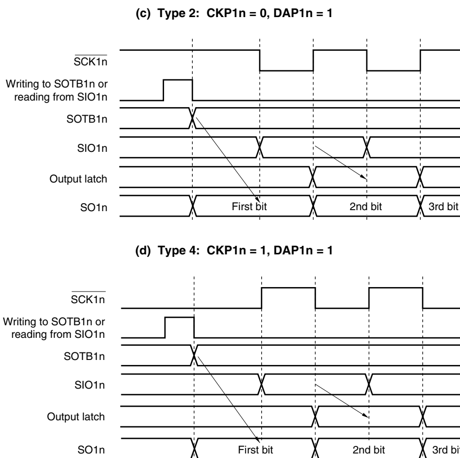
Figure 16-17. Output Operation of First Bit (2/2)
