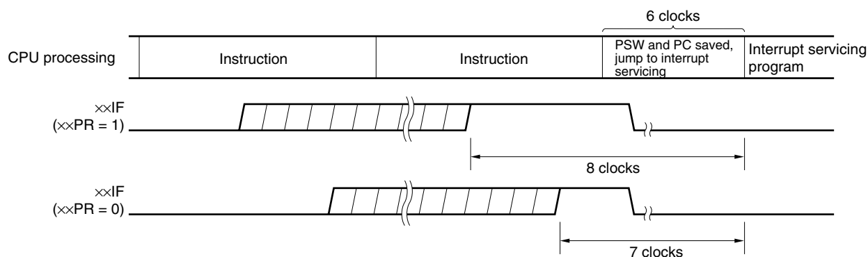
Figure 17-26. Interrupt Request Acknowledgment Timing (Minimum Time)
