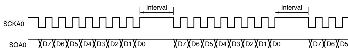
Figure 17-20. Example of Repeat Transmission Mode Operation Timing
