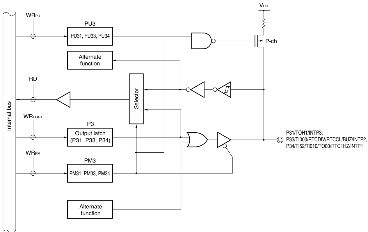
Figure 4-9. Block Diagram of P31, P33, P34
