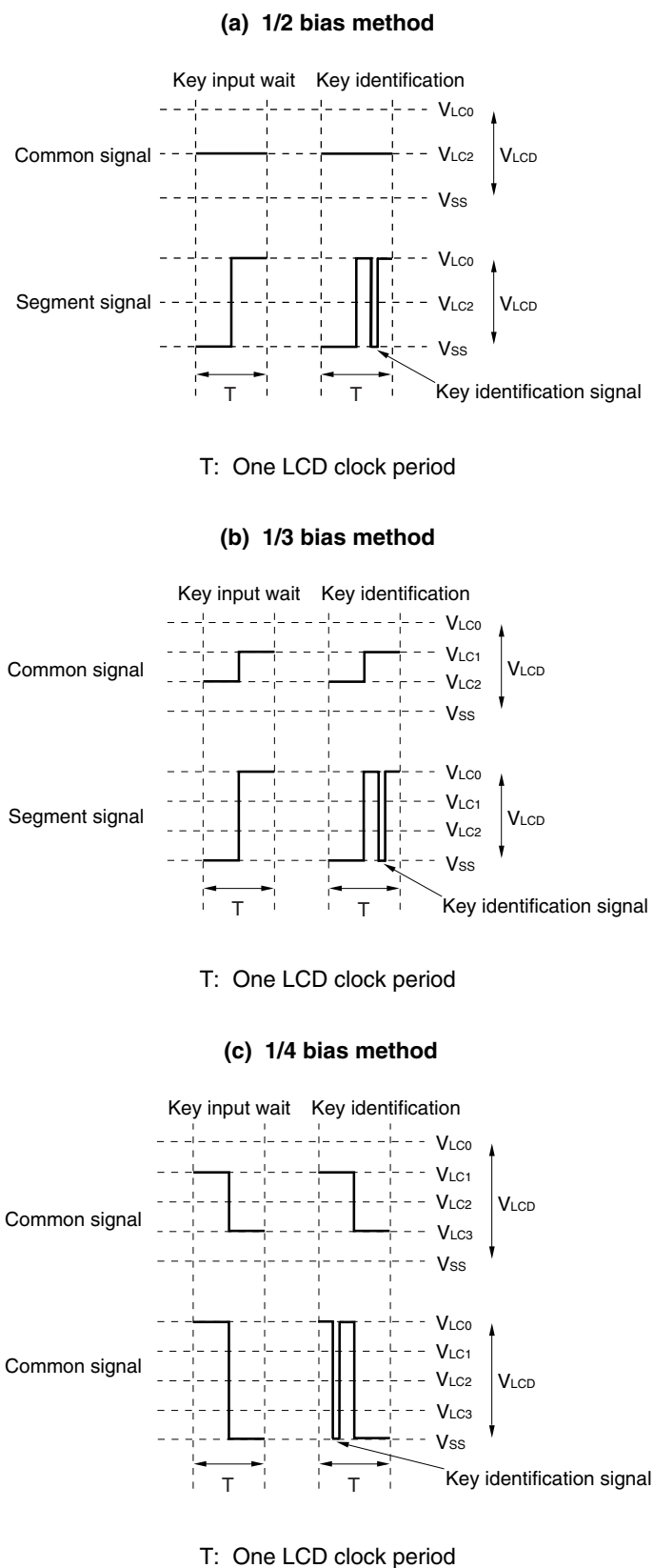
Figure 18-19 Voltages and Phases of Common and Segment Signals
