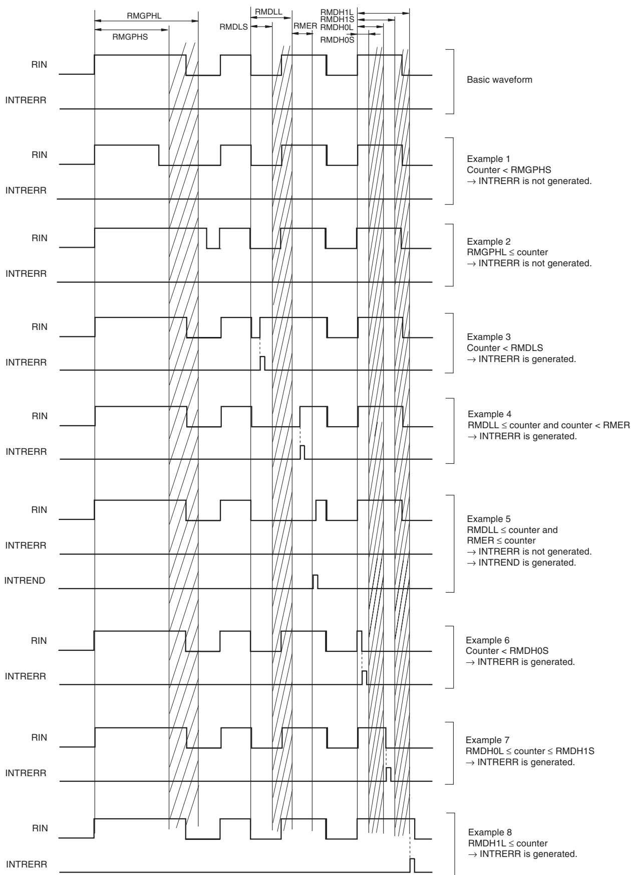
Figure 20-13. Generation Timing of INTRERR Signal (Type A reception mode)
