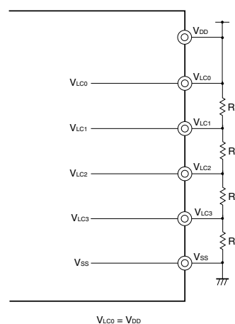
(g) 1/4 bias method (MDSET1, MDSET0 = 0, 0) (example of V_{DD} = 5\text{ V} , V_{LC0} = 5\text{ V} )
