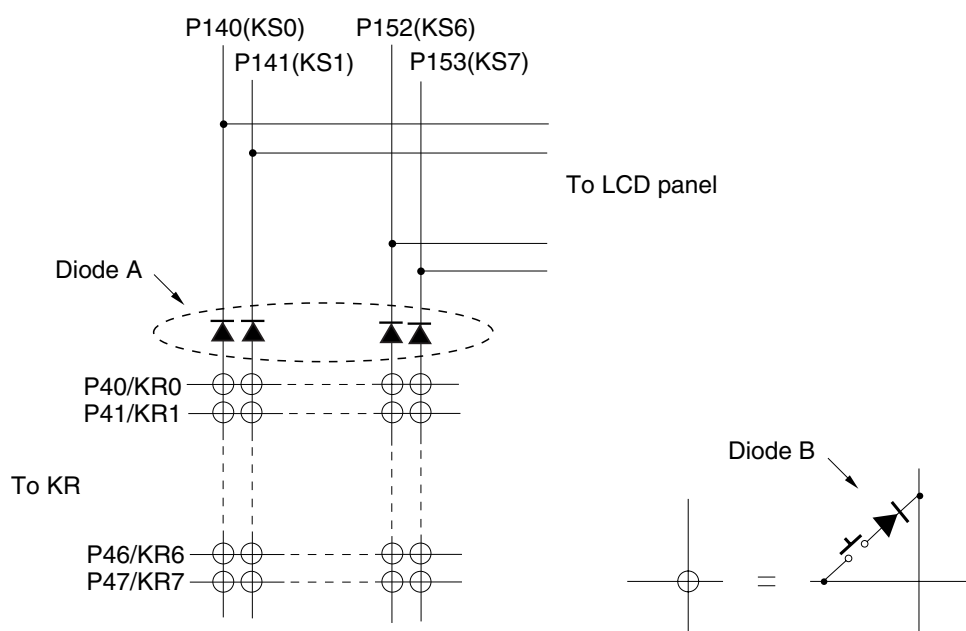
Figure 18-41. Key Matrix Configuration Example (78K0/LF3)
