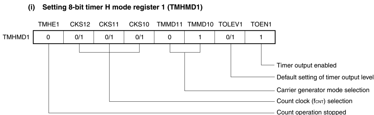
Figure 8-16. Register Setting in Carrier Generator Mode
